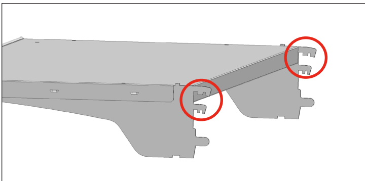
Fig. 21. Angle adjustment slots on the shelf support.
