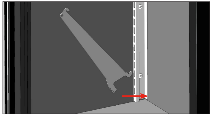
Fig. 6. Hook the shelf support into the shelf standard.
