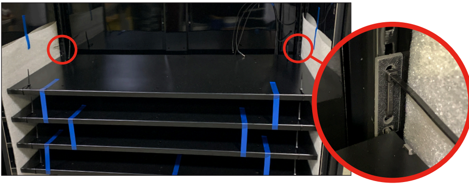
Fig. 18. Shelf shipping brackets located in the shelf standards above the shelf.
