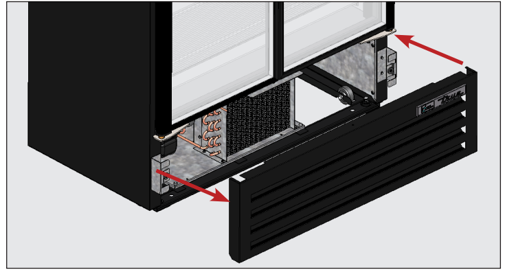
Fig. 2. Carefully remove the grill.
