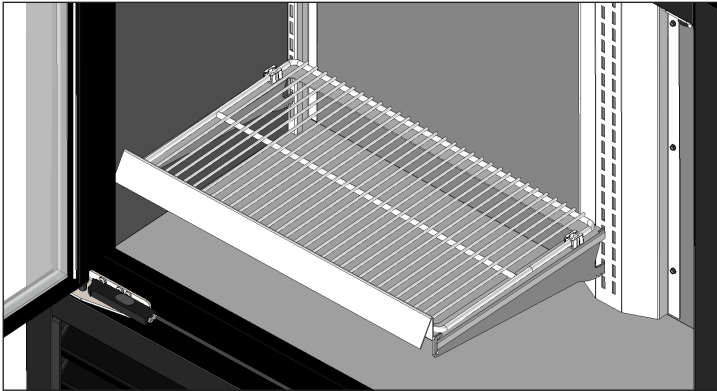
Fig. 17. Installed wire cantilever shelf.
