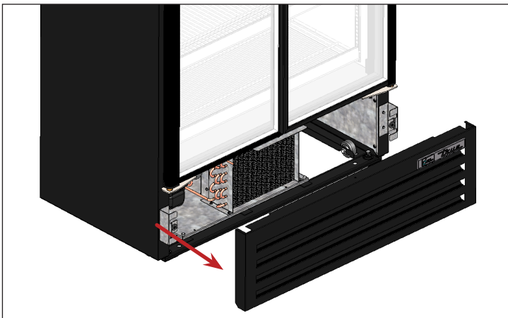
Fig. 3. Carefully remove the grill from its magnets.
