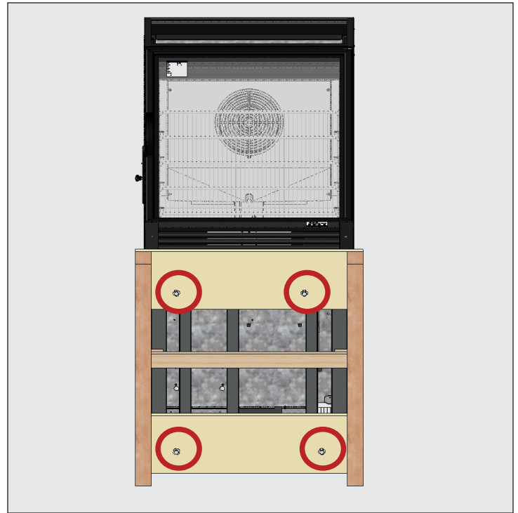
Fig. 4. Shipping bolt locations.
