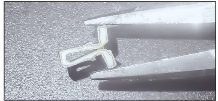
Fig. 10. Squeeze the hinge retention clip.
