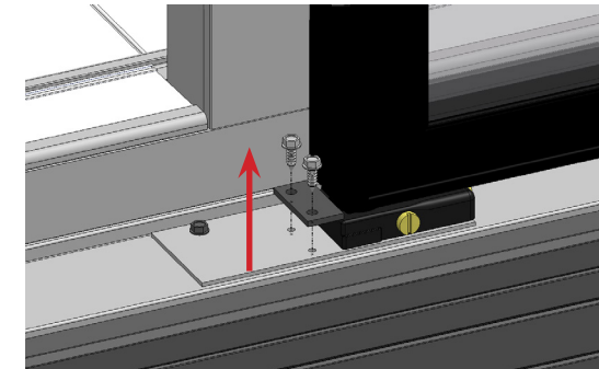
Fig. 1. Remove the door shipping plate.
