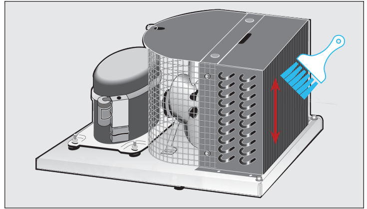
Fig. 2. With a stiff bristle brush clean off accumulated dirt from the condenser coil.
