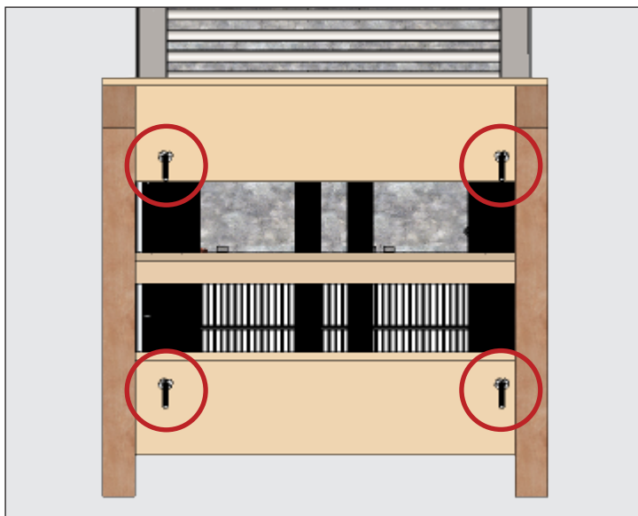
Fig. 3. Shipping bolt locations.
