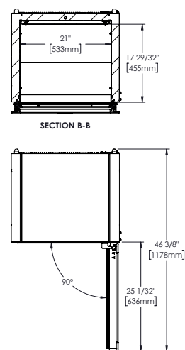
Top View
