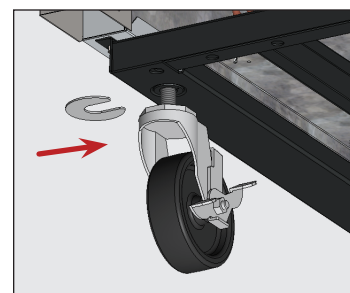
Fig. 9. Insert the castor shim(s). be sure to tighten the castor stem.
